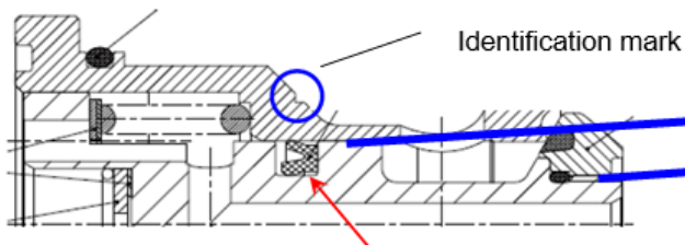
Exhaust cartridge ED07 (E ED07)
