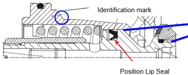
Exhaust cartridge ED12 (E ED12)
