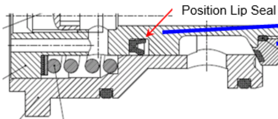
Supply cartridge ED07 (S ED07)
