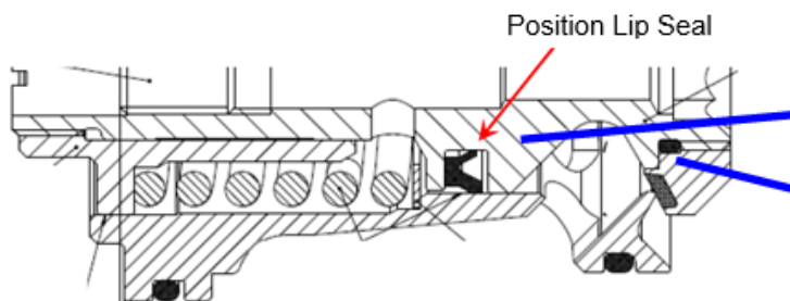
Supply cartridge ED12 (E ED12)
